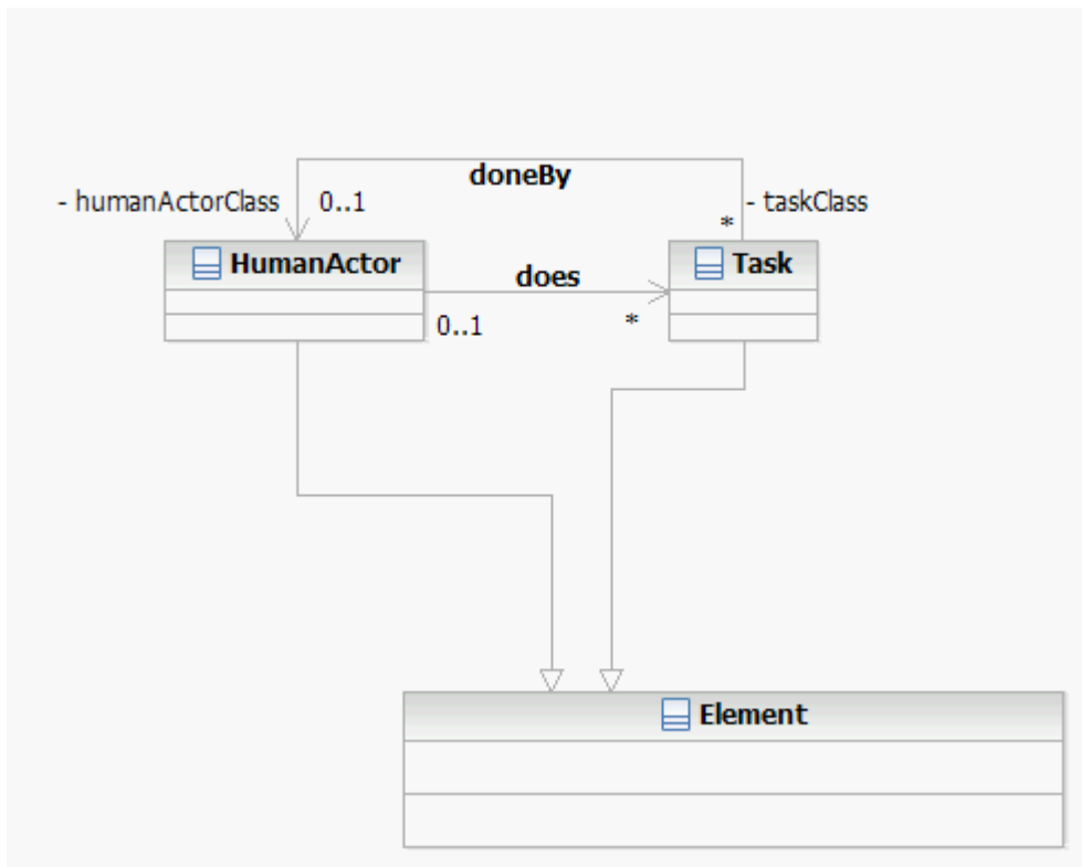
Figure 7: The Task Class
