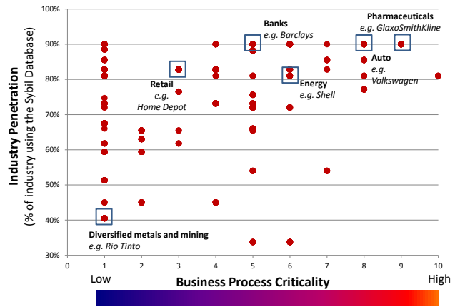
Figure 7: Industry sector scoring (GCIS Sub-industry classification) of penetration and criticality by sector
