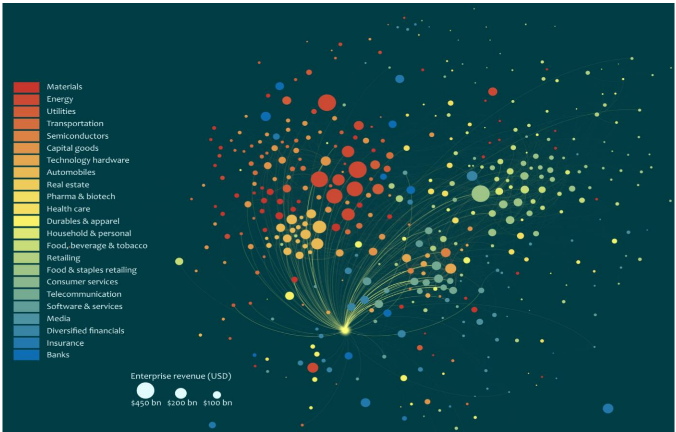
Figure 6: Mapping the Cyber Economy: 600 companies by GICS industry group.
